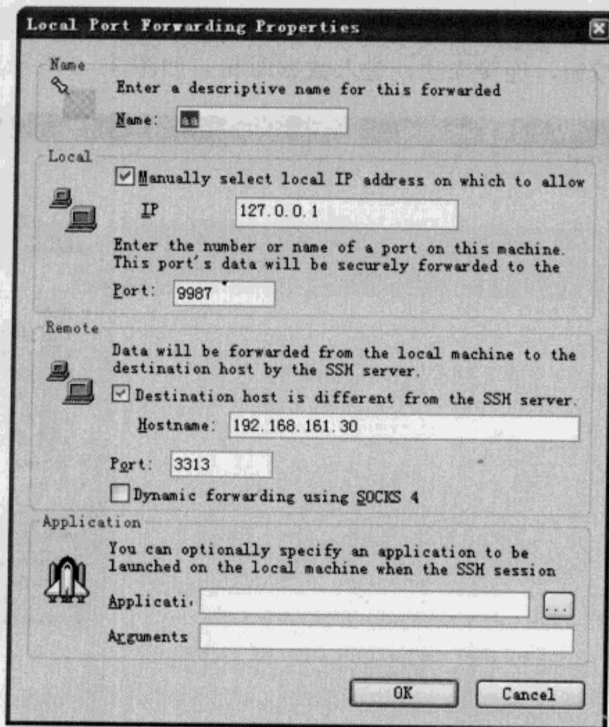
图 31-4 “Local Port Forwarding Properties”对话框
