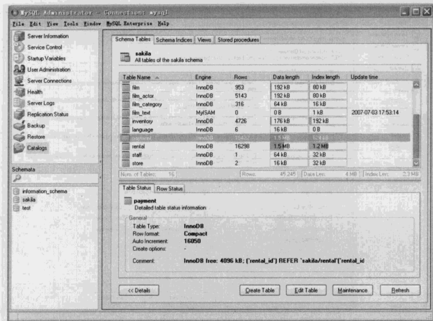
图 6-6 MySQL Administrator Catalogs
